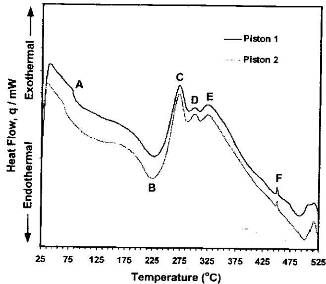
Fig. 5 DSC curves during heating of the as-quenched Al-Si piston alloys
