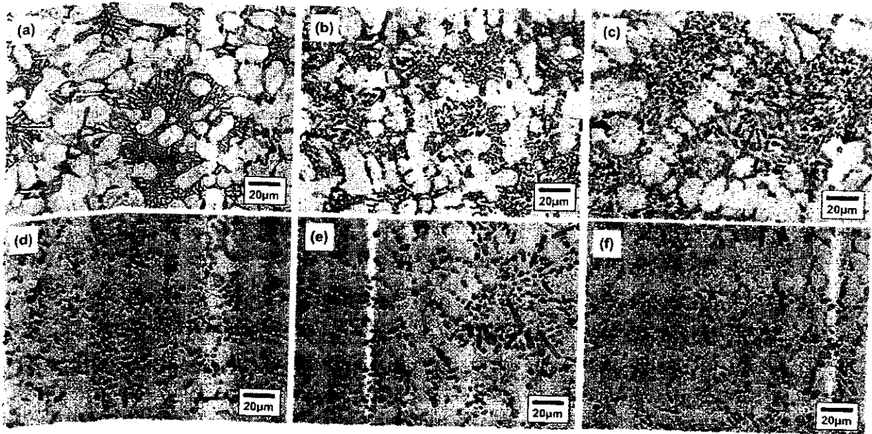
Fig. 2 Microstructure of the piston 1 with various conditions; (a) as-cast, (b) 0.5 h (c) 2 h, (d) 4 h, (e) 6 h and (f) 10 h solution treatments, respectively.
