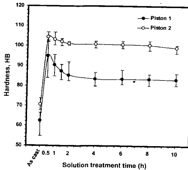
Fig. 4 Evolution of hardness value as a function of the solution treatment times.
