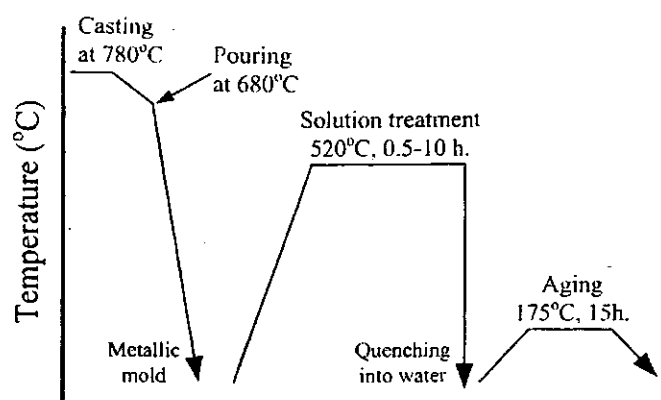
Fig. 1 Schematic illustration of experimental procedure.
